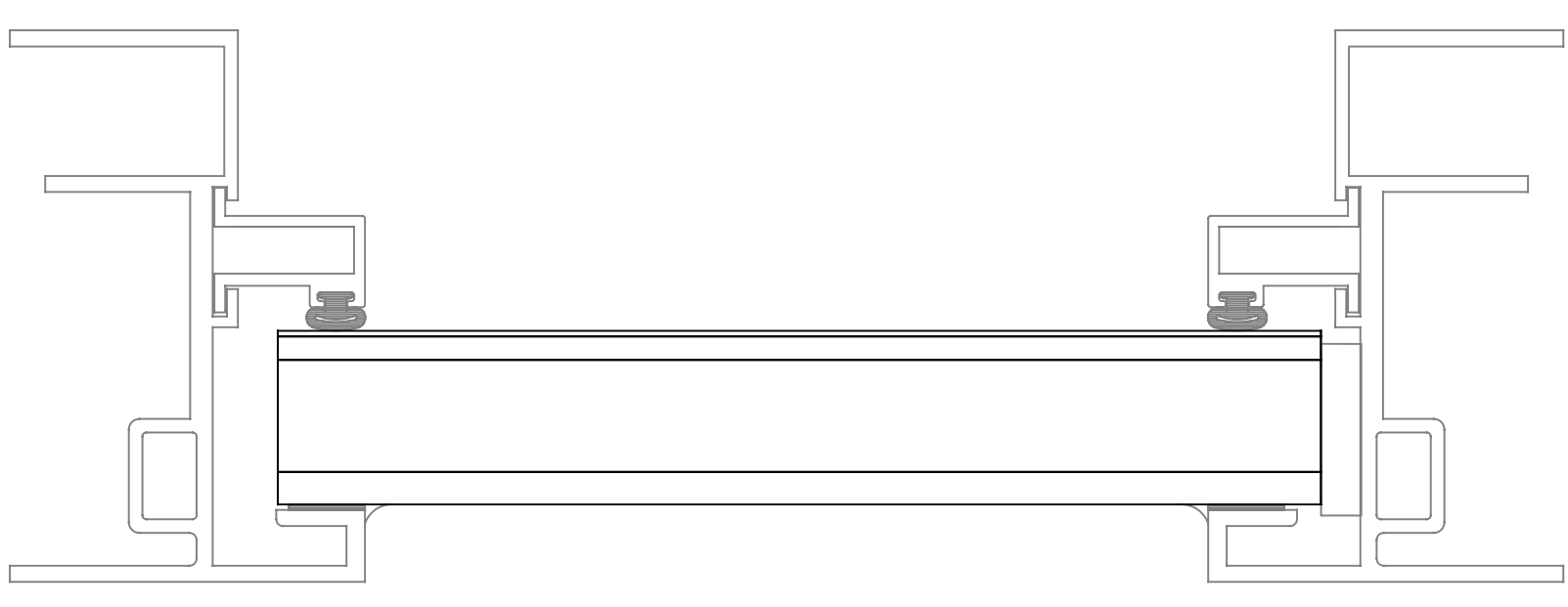
WINDOW FRAME
