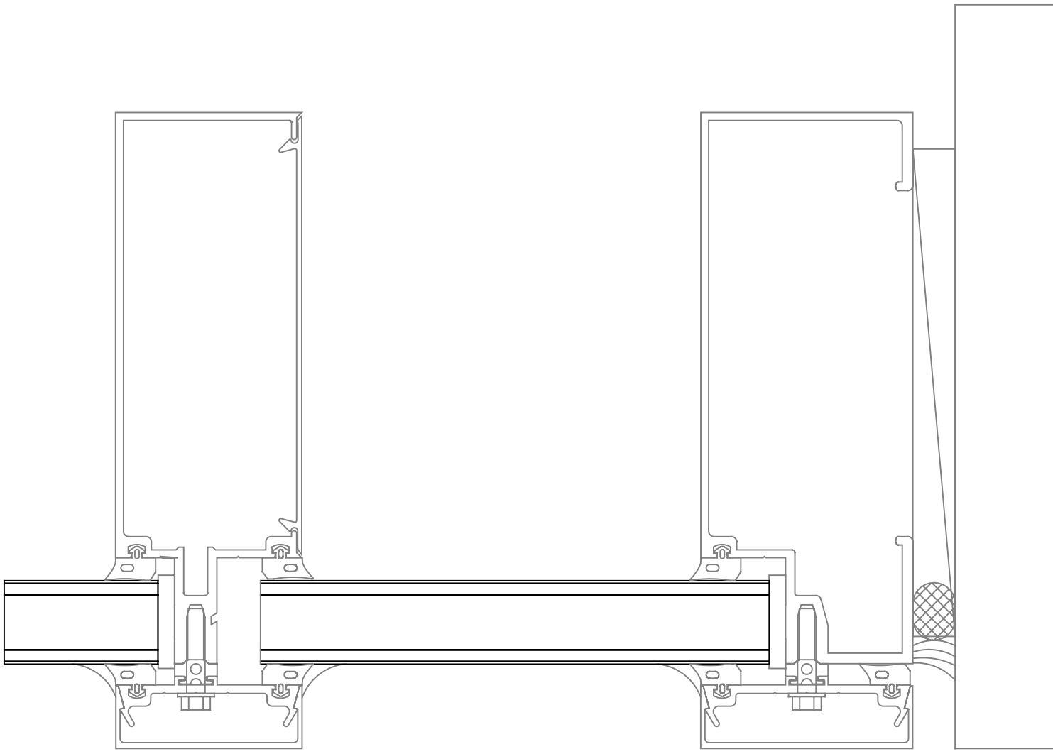
CURTAIN WALL
