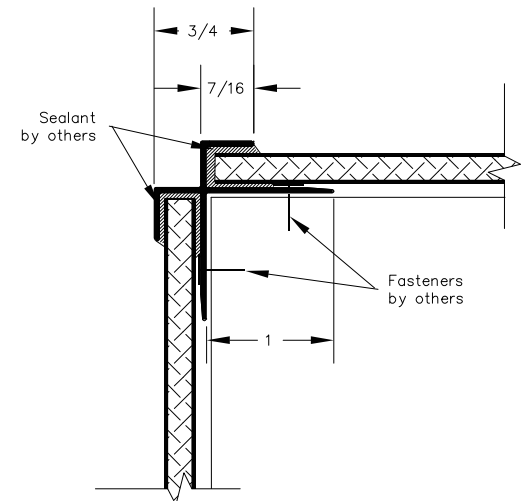
Outside corner MIN-41
